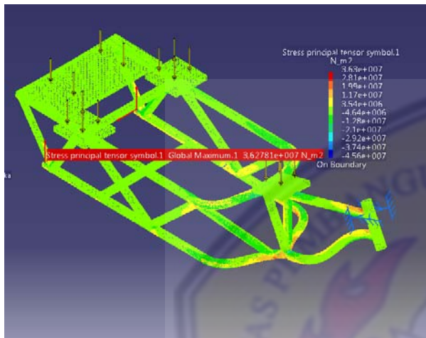
Gambar 14 Tegangan Principal Tensor
